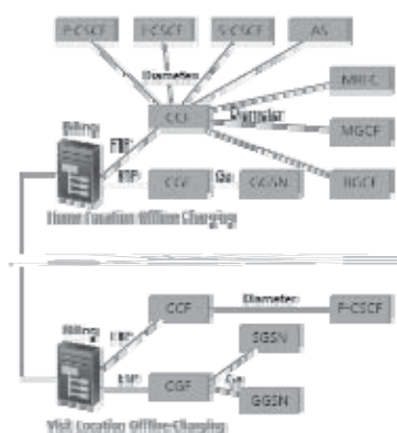
Fig.2 Offline charging
