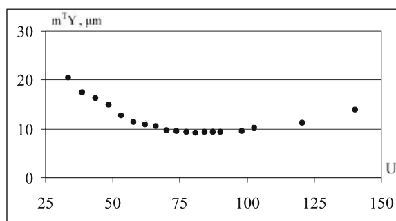
Fig. 5. Influence of the angle of photogrammetric intersection on accuracy of coordinates received on quasi-stereo mate
