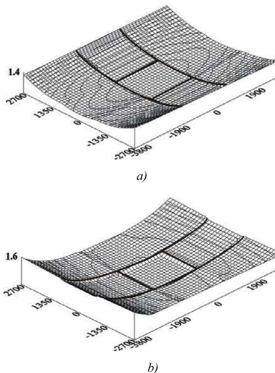
Fig. 2. The values of the errors on the quasi-snap (3 points at the strip of overlapping): a) on axe X; b) on axe Y
