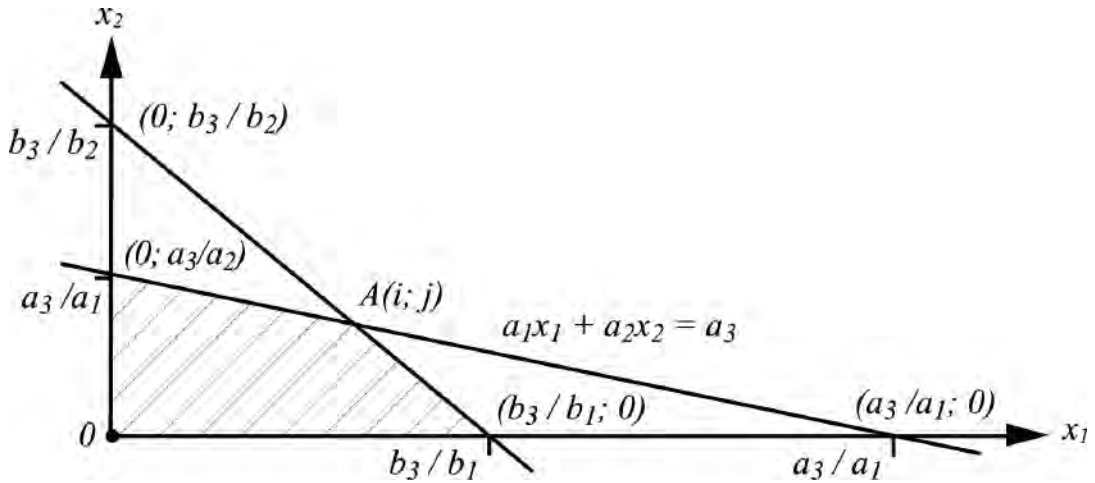
Fig. 4. Solution of the system of inequalities (1)
