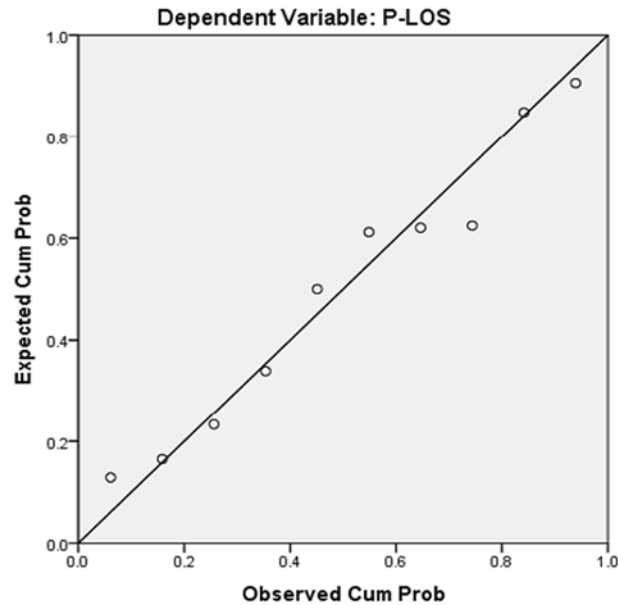
Fig. 2. Normal P-P Plot of Regression Standardized Residuals
