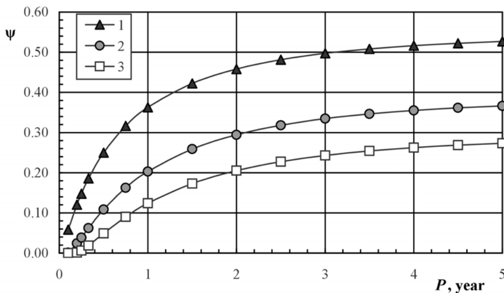
Fig. 3. Daily runoff coefficient \psi for pervious surfaces of the city of Lviv as a function of the return period P for soils of hydrologic group C: 1) poor condition; 2) fair condition; 3) good condition
