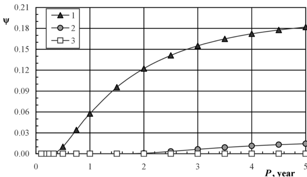
Fig. 1. Daily runoff coefficient \psi for pervious surfaces of the city of Lviv as a function of the return period P for soils of hydrologic group A: 1) poor condition; 2) fair condition; 3) good condition
