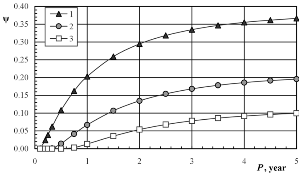
Fig. 2. Daily runoff coefficient \psi for pervious surfaces of the city of Lviv as a function of the return period P for soils of hydrologic group B: 1) poor condition; 2) fair condition; 3) good condition
