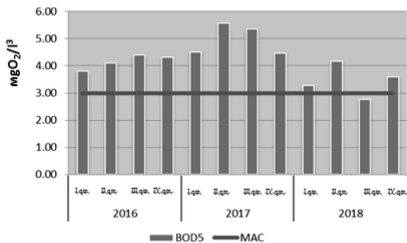
Fig. 7. Dynamics of changes in concentrations of \text{BOD}_5 at the observation point of the Poltva River – Kamianka-Buzka
