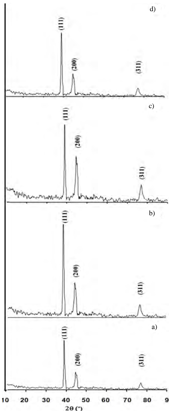
Fig. 3. X-ray diffraction pattern of silver nanoparticles prepared by discharge plasma at different concentrations of PVP (%): 0.5 (a); 1.0 (b); 1.5 (c) and 2.5 (d)
