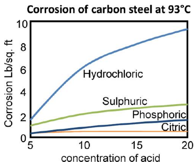
Fig. 3. Dependence of corrosion on concentration of some acids (Hogendoorn, 2016).
