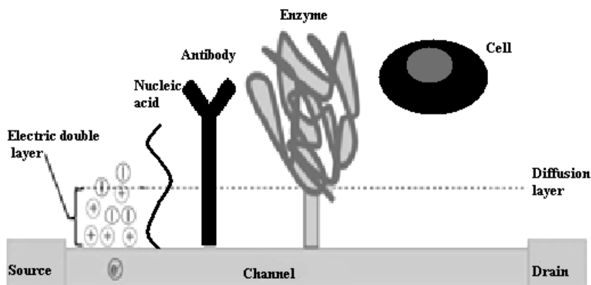
Fig. 3. Schematic image of the sensitive area of the ISFET and assays with different sizes in relation to the thickness of the electric double layer
