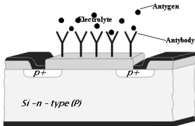
Fig. 4. Schematic structure of immune-ISFET with antibodies
