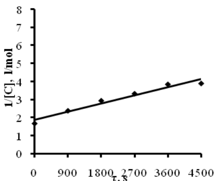
Fig. 2. Kinetic anamorphoses in coordinates 1/[C_{carb.gr.}] - \tau for the reaction of DPPDE with DABCO at 343 K in isopropyl alcohol medium. The amount of DABCO is 20 mol % per 1 g-eq. of DPPDE epoxy group
