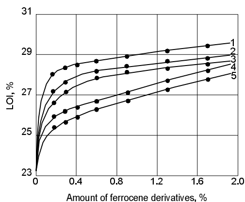
Fig. 10. Dependence between LOI of epoxy matrix mortars and amount of ferrocene derivatives: α-oxethylferrocene (1); ferrocene (2); diacetylferrocene (3); ferrocenedicarboxylic acid (4) and acetylferrocene (5)
