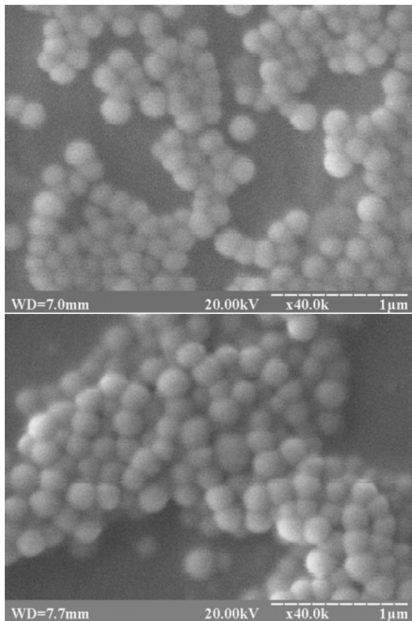
Fig. 2. SEM micrographs of \text{SiO}_2 NP obtained in presence of 5 % (a) and 50 % (b) RC-3 with respect to \text{SiO}_2 weight ( T=303 K, C_{\text{H}_2\text{O}}=25 mole/l, C_{\text{NH}_4\text{OH}}=5 mole/l)
