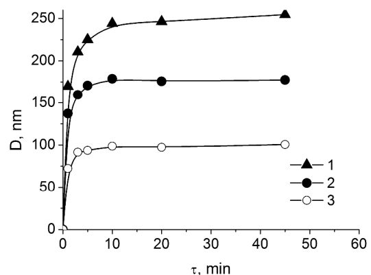
Fig. 4. Kinetics of \text{SiO}_2 NP growth in presence of 5 % RC-4 depending on \text{H}_2\text{O} concentration: C_{\text{H}_2\text{O}}=20 mole/l (1), 25 mole/l (2), 30 mole/l (3) ( T=303 K, C_{\text{NH}_4\text{OH}}=2,5 mole/l)
