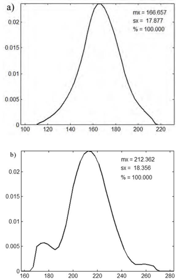
Fig. 3. Curves of size distribution of \text{SiO}_2 NP obtained in the presence of 5 % (a) and 50 % (b) RC-3 with respect to \text{SiO}_2 weight ( T=303 K, C_{\text{H}_2\text{O}}=25 mole/l, C_{\text{NH}_4\text{OH}}=5 mole/l)
