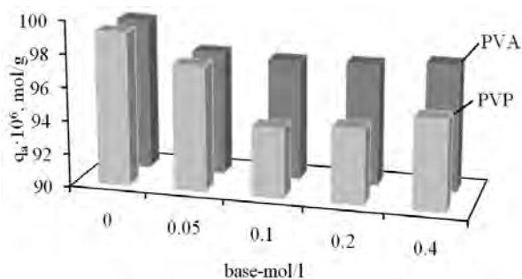
Fig. 2. Influence of nature and concentration of polymer modifier on the number of active centers of Ni-PSM
