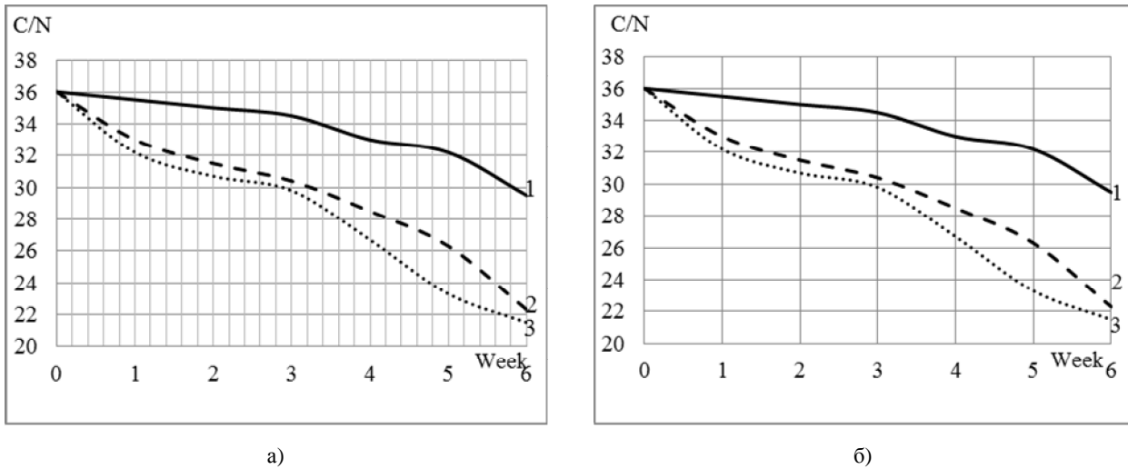
Fig. 8. Dynamics of change in C/N during composting with mineral (a) and microbiological (b) additives in mesophilic (2) and thermophilic modes (3) as compared to the control sample (1)
