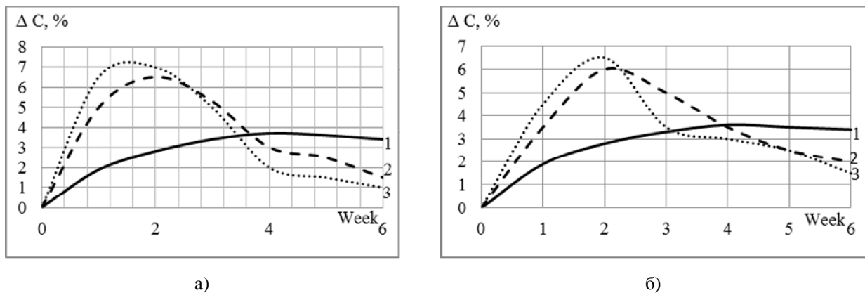
Fig. 6. Change in the total Carbon during the composting process with mineral (a) and microbiological (b) additives in mesophilic (2) and thermophilic modes (3) as compared to the control sample (1)
