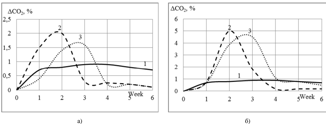
Fig. 5. Change in CO 2 emissions during the composting process with mineral (a) and microbiological (b) additives in the mesophilic (2) and thermophilic regimes (3) as compared to the control sample (1)
