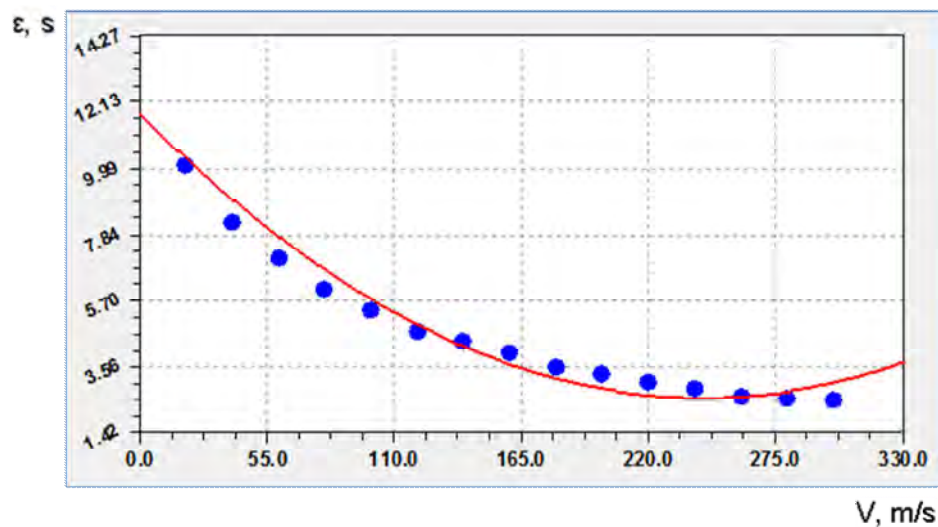
Fig. 3. Experimental (●) and polynomial calculated (—) thermal response time depending on gas flow velocity.
