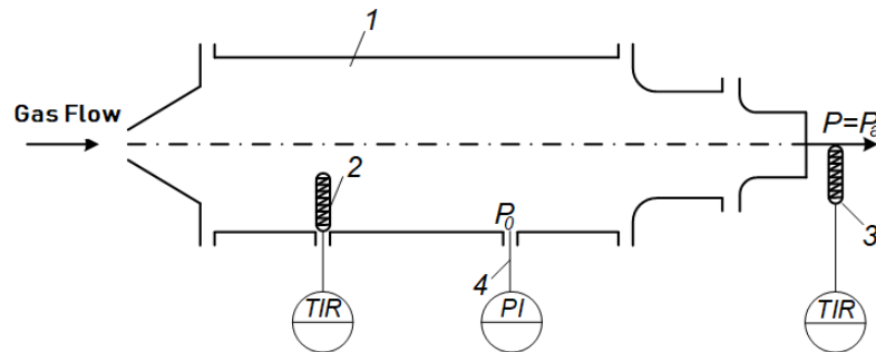
Fig. 2. Scheme of the measuring unit for determining the time of thermal reaction: 1 – wind tunnel with open working part; 2 – platinum resistance thermocouples for measuring the temperature in the wind tunnel; 3 – investigated thermo transducer; 4 – pressure gauge for measuring full pressure.
