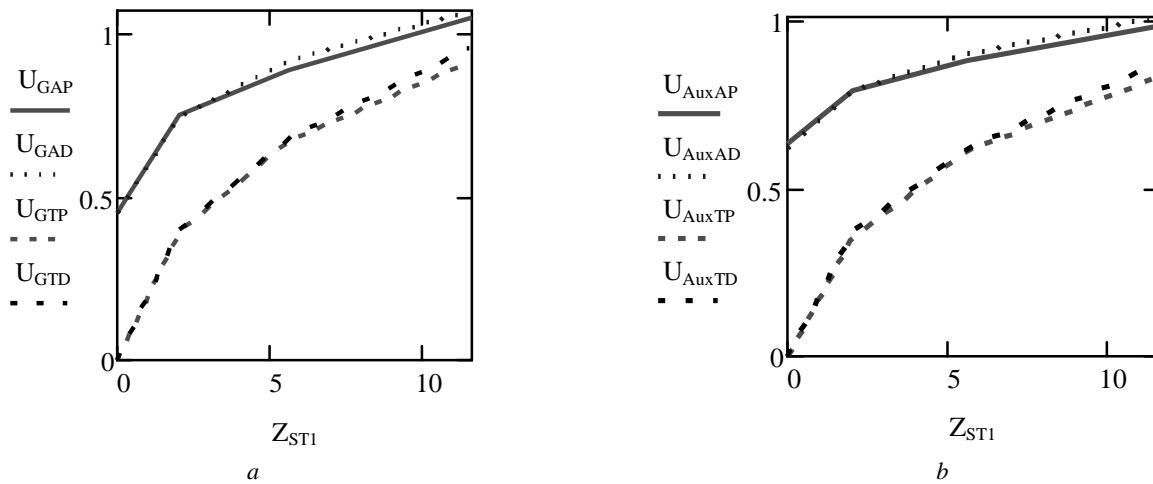
Fig. 3. Voltage dependence for digital (D) and physical (P) scheme models of the PU with an AAT(A) and a traditional scheme of the PU without an AAT (T) from resistance Z_{ST1} : a - U_G^* ; b - U_{Aux}^* .
