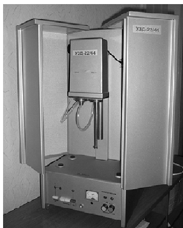
Fig. 1. Ultrasonic generator UZDN-2T for combustion of organic matters inclusions and microorganisms disinfection in the ultrasonic field
