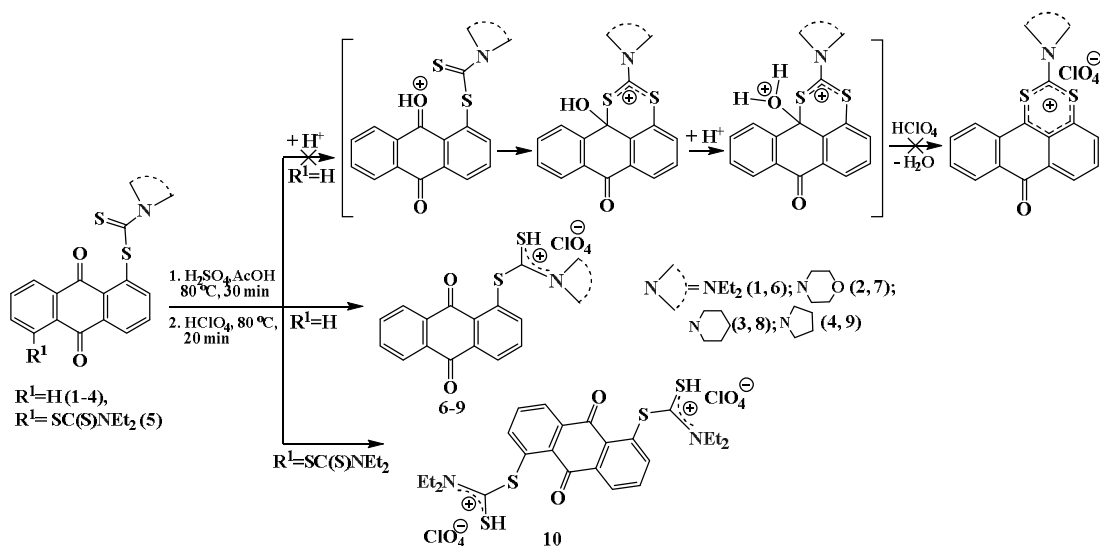
Scheme 1. Obtaining of the perchlorates 6-10
