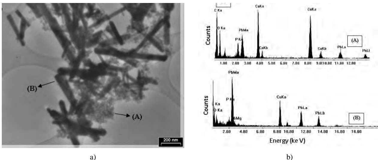
Fig. 8. TEM micrograph (a) and EDS spectrum of \text{Pb}^{2+} -loaded the nano hydroxyapatite granules sample after adsorption (b)
