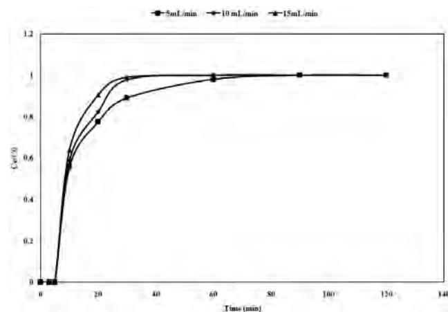
Fig. 3. Breakthrough curves expressed as C_e/C_0 vs. time at different flow rates (lead initial concentration 500 mg/l, initial pH 7.5, bed depth 10 mm and temperature 298 \pm 1 K)
