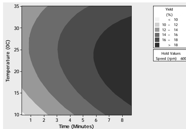
Fig. 4b. Contour plot of temperature (B) against time (A)
