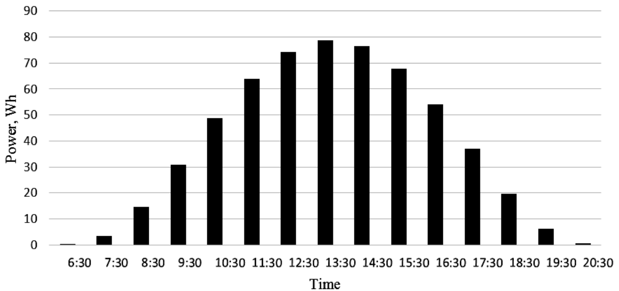
Fig. 5. Estimation of the produced amount of electricity
