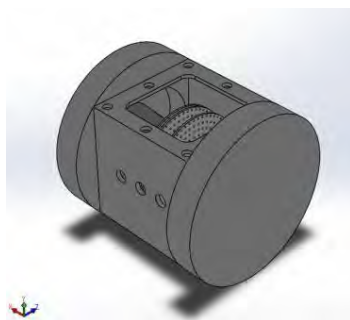
Fig. 4. SolidWorks 2016 Educational solid-state model – complete assembly of the working chamber with three cavitation disks
