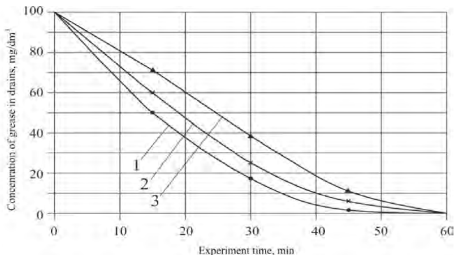
Fig. 6. Dynamics of changes in the time of concentration of technological grease in contaminated water with the use of adsorbent of different granulometric composition (mm): 1 – 0,03–0,01 mm; 2 – 0.1–1.0; 3 – 1.0–3.0
