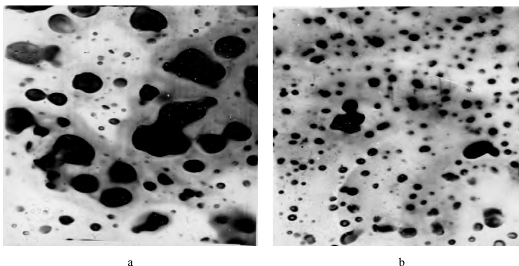
Fig. 4. Results of electron microscopic study of buckwheat husk briquette adsorbent (6700 times increased) at different stages of its production: a – raw material grinding and interaction with sulphate acid; b – mechanical and chemical activation
