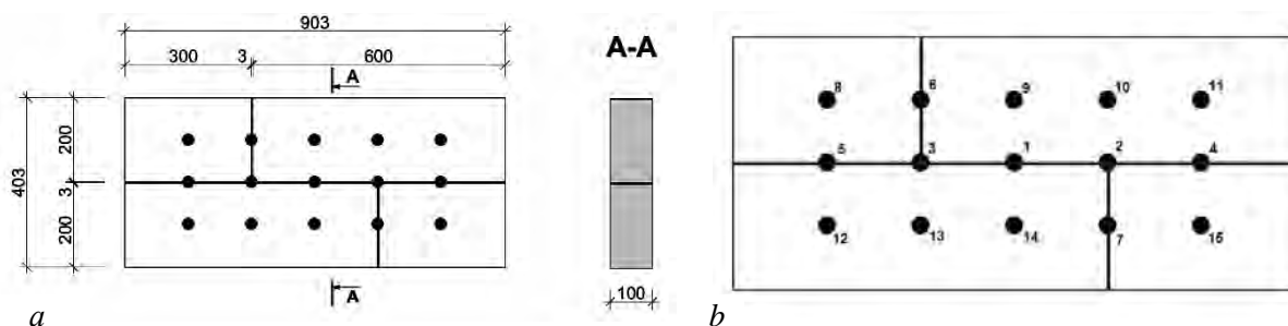
Fig. 2. Shape of test masonry specimens (a) and drilling order (b)
