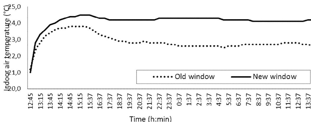
Fig. 1. The measured indoor air temperature
