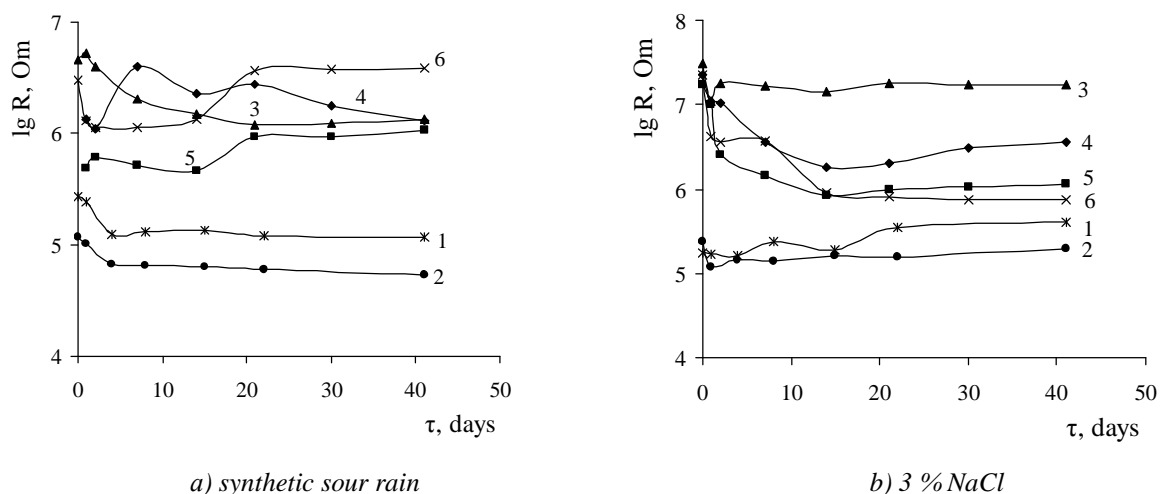
Fig. 3 Change of logarithm of electrical resistance of polyester coatings over time. PVC content, wt. p.: 1-0; 2, 4-6 – 10; 3 – 20. \text{CaCO}_3 content, wt. p.: 1-4, 6 – 0; 5 – 25. \text{Al}_2\text{O}_3 content, wt. p.: 1-5 – 0; 6 – 25; DBF content, wt. p.: 1-3, 5, 6 – 0; 4 – 3
