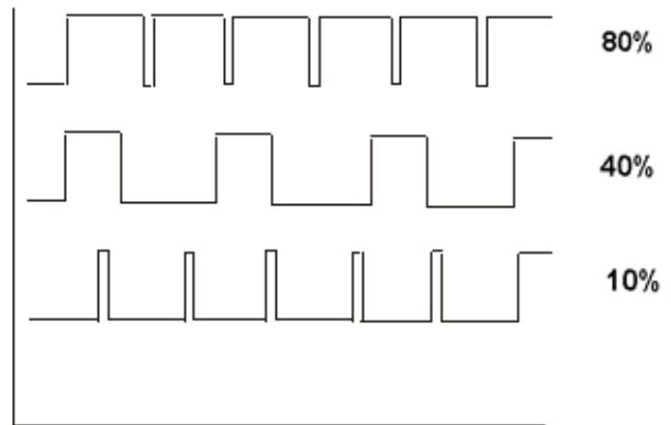
Fig. 5. Width-pulse modulation
