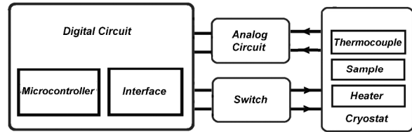
Fig. 1. Block diagram of automated installation
