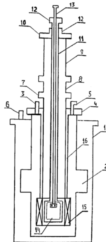
Fig. 2. Design of the cryostat: 1 – helium cryostat; 2 – volume for liquid helium; 3, 6 – the inlet pipes; 4, 7, 10 – flanges; 5 – outlet pipe; 8 – vacuum valve; 9 – gateway, 11 – holder; 12 – clamping device; 13 – push-type actuator; 14 – cryostat and sample; 15 – heater
