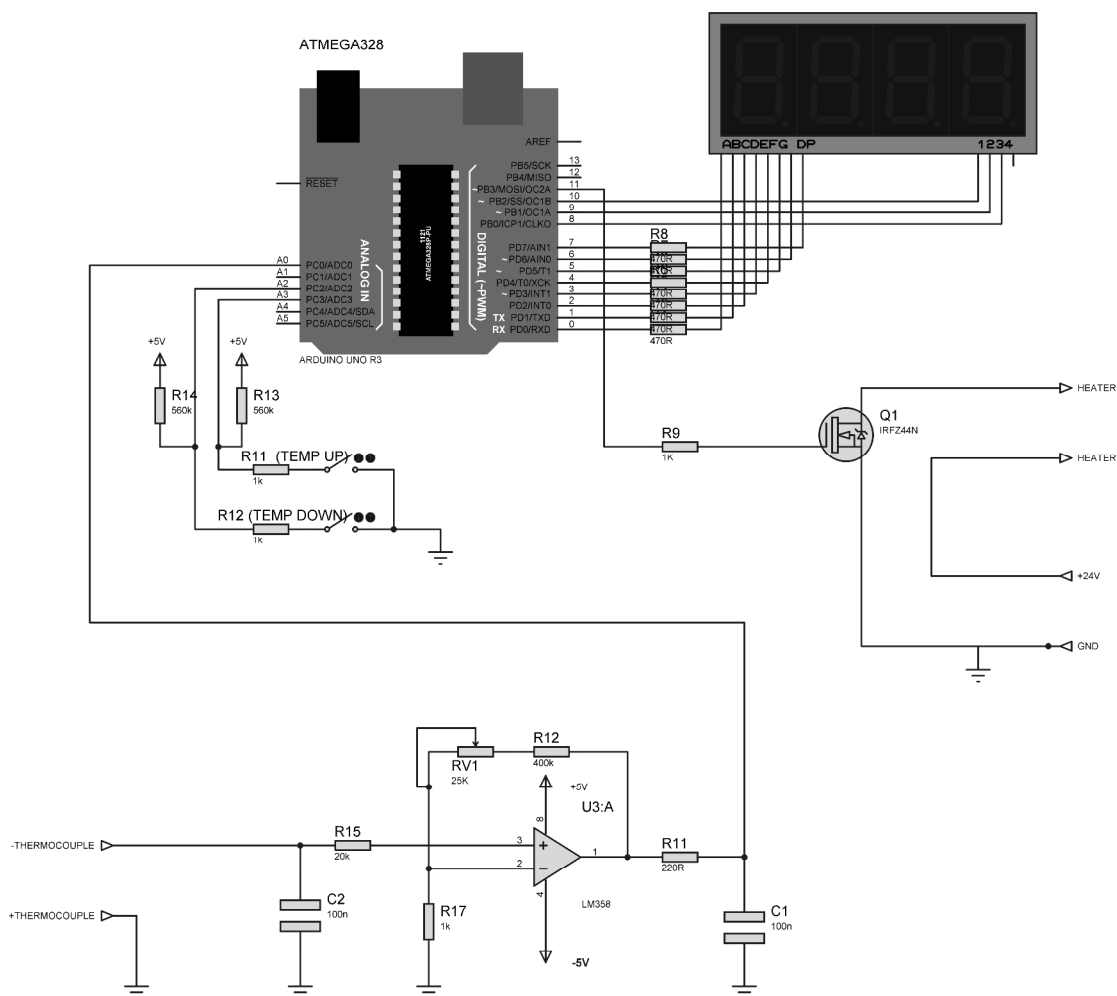
Fig. 3. Electronic diagram of the thermostat heater controller
