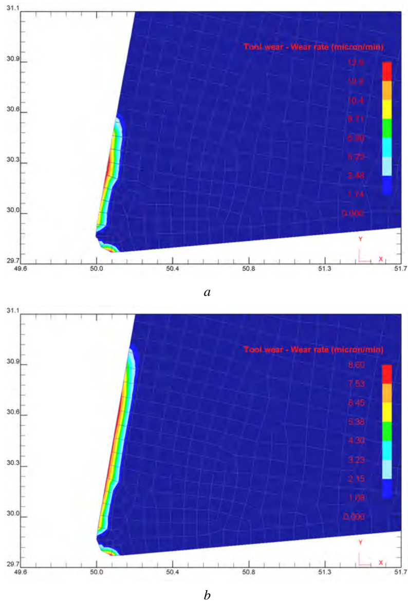
Fig. 8. Results of unhardened ( a ) and hardened by ADH method ( b ) tool wear rate modeling for the workpiece's machining made of steel AISI 45 (cutting modes: cutting speed V = 158.3 m/min, feed per tooth S = 0.12 mm, depth t = 1.0 mm)
