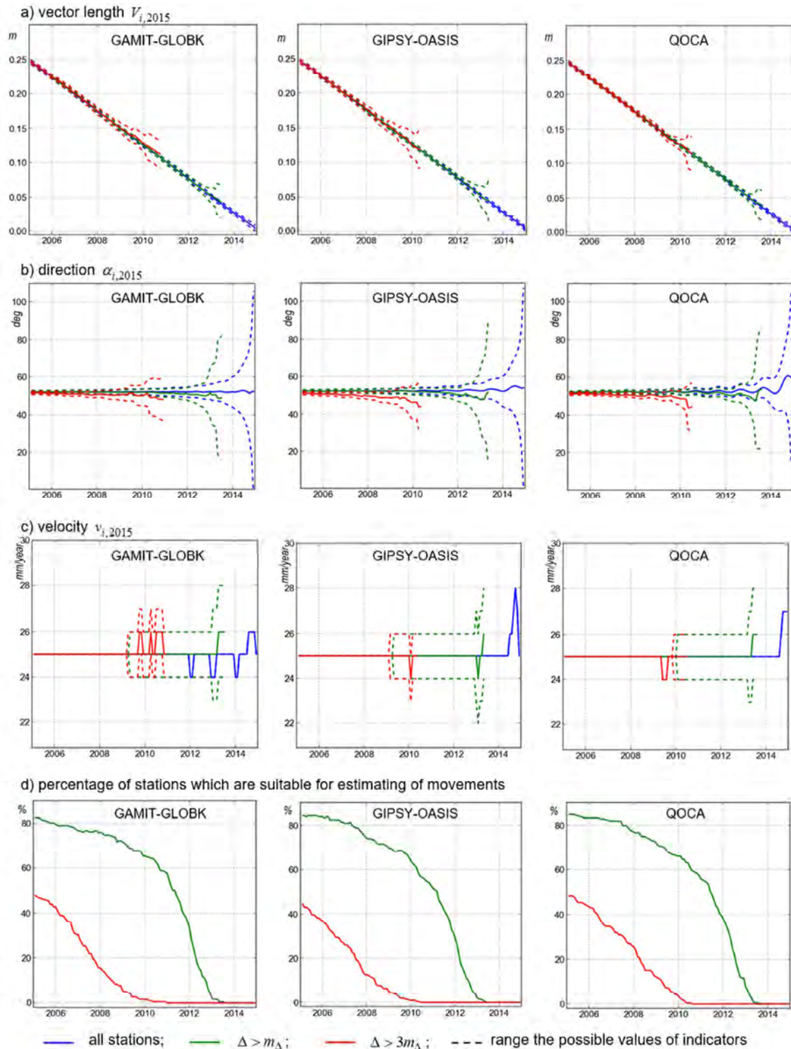
Fig. 2. Average motion parameters of the Earth's surface 2005–2015
