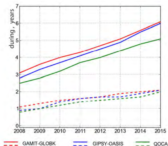
Fig. 4. Minimum duration of observational periods sufficient to achieve the parameter accuracy of the millimeter (solid lines) and centimeter level (dotted lines)
