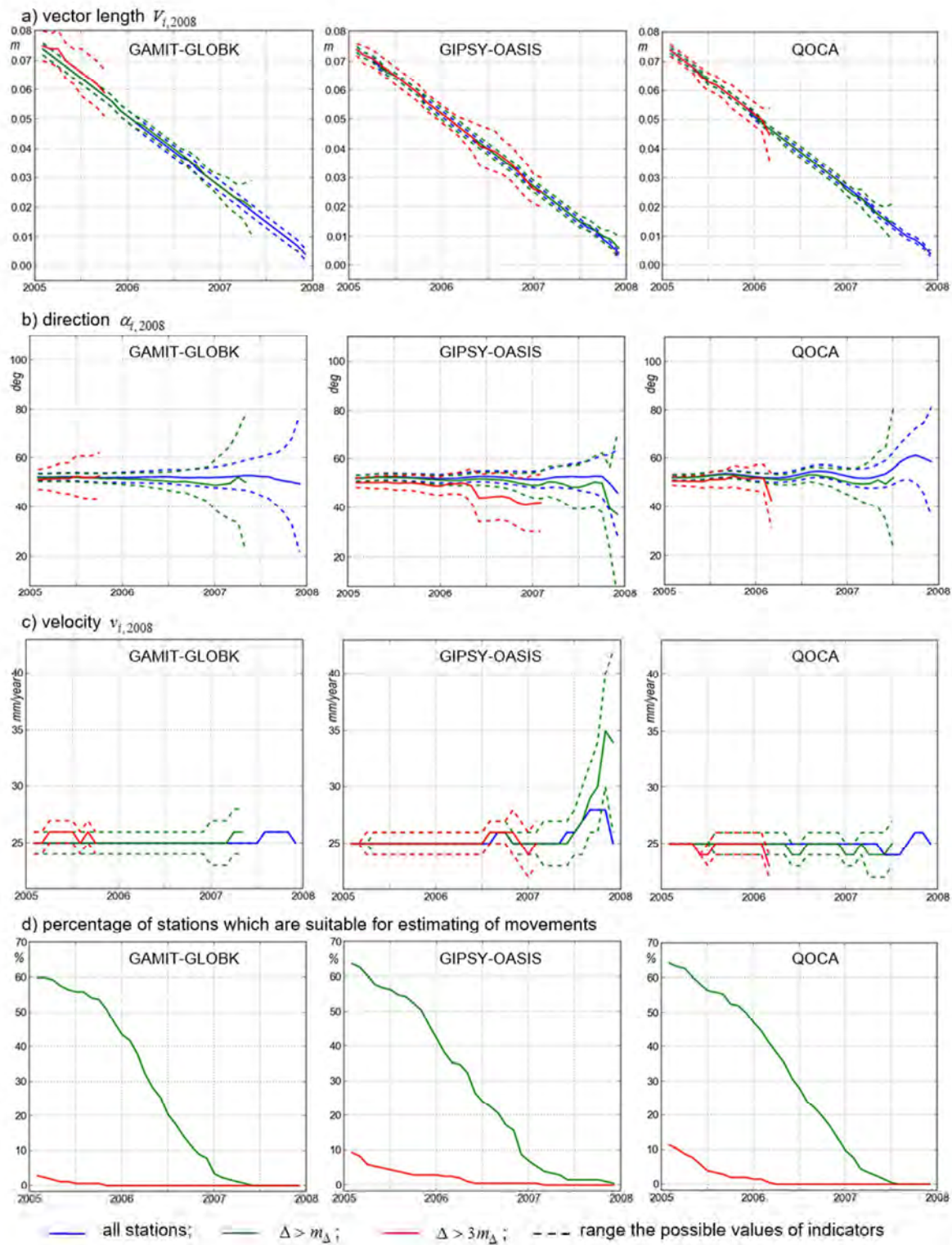
Fig. 3. Average motion parameters of the Earth's surface 2005-2008
