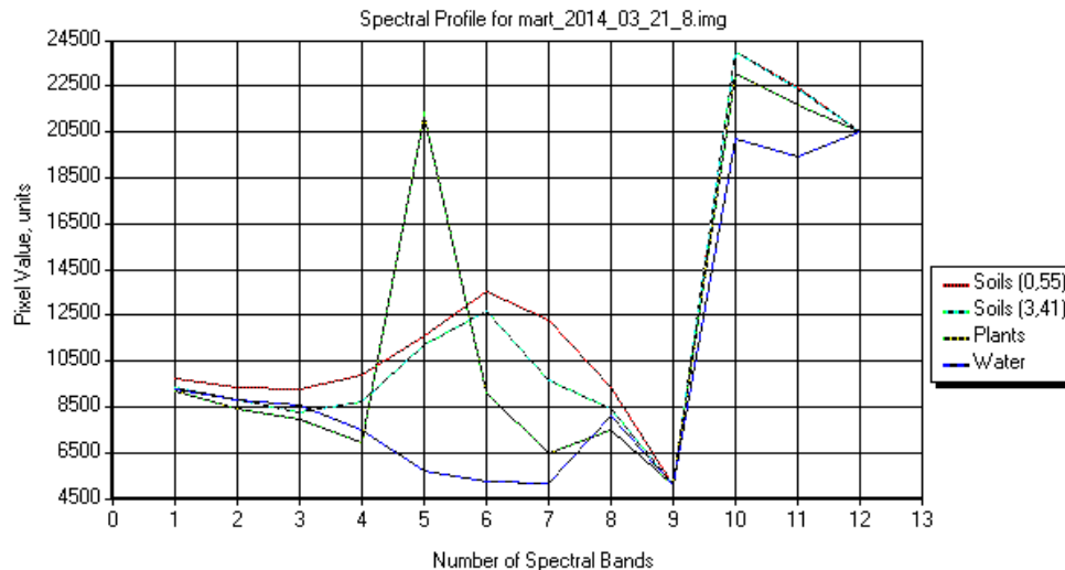
Fig. 1. Spectral profiles of soil, plants, and water according to Landsat 8 OLI
