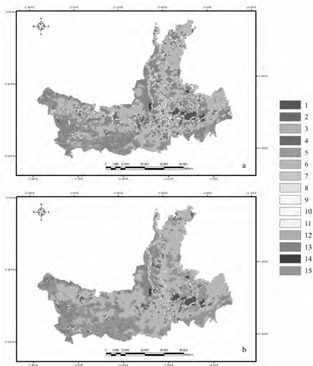
Fig. 2. Output classifications of the land cover (MCD12Q product) on WP TBR territory: a – 2001, b – 2013. IGBP classes: 1 – water bodies; 2 – evergreen needleleaf forest; 3 – evergreen broadleaf forest; 4 – deciduous needleleaf forest; 5 – deciduous broadleaf forest; 6 – mixed forest; 7 – closed shrublands; 8 – open shrublands; 9 – woody savannas 30–60 %; 10 – savannas 10–30 %; 11 – grasslands; 12 – permanent wetlands; 13 – croplands; 14 – urban and built-up lands; 15 – cropland/natural vegetation mosaics
