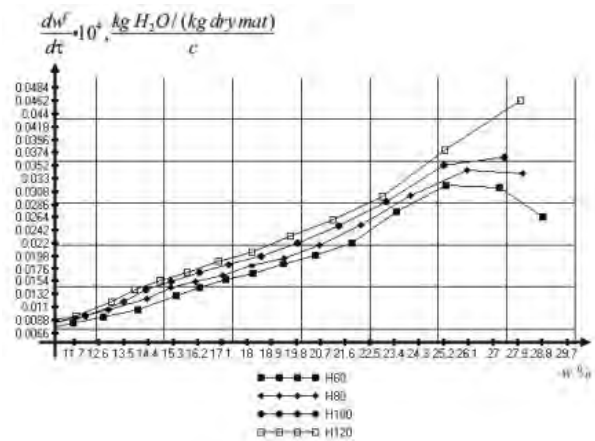
Fig. 4, d. The filtration dryingspeed by different heights of the layer ( v_0 = 1,38 \text{ m/s} , T = 70 \text{ }^\circ\text{C} )
