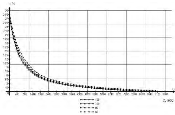
Fig. 4, b. Change of the moisture layer of buckwheat in time by different heights of the layer ( v_0 = 1,38\text{m/s} , T = 70 \text{ }^\circ\text{C} )
