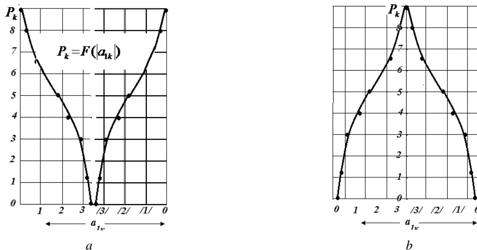
Fig. 3. Graphical solution for transformation of the functional \mathcal{R}_{P_k} = f[P_k] for the reversed problem P_k = F(|a_k|)
