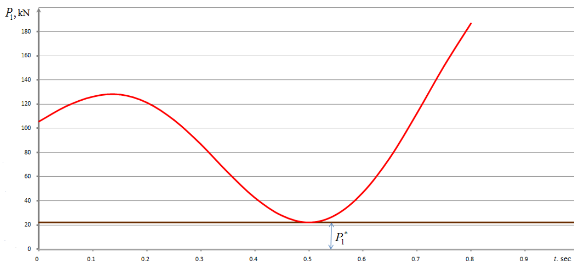
Fig. 4. The plot for checking the necessary condition of the wheelset rolling onto the rail head at u = 37 \text{ km/h} , h = 0.0213 \text{ m}
