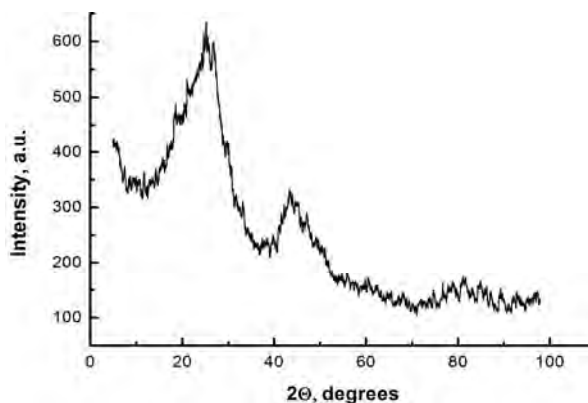
Fig. 2. The diffractogram of the activated carbon made of sugar beet pulp
