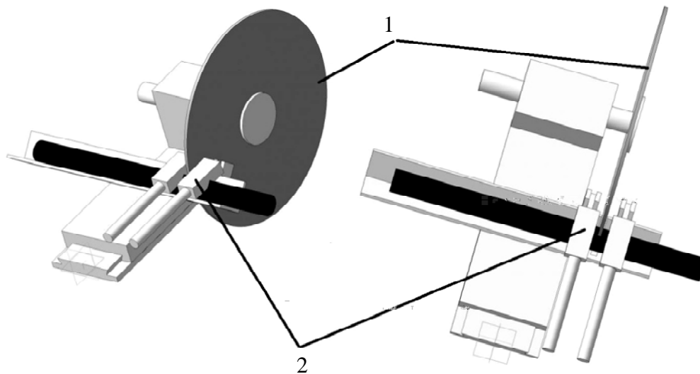
Fig. 6. Scheme of HPH fixing (clamping) with regard to cutting disc: 1 – cutting disc; 2 – hose fixers
