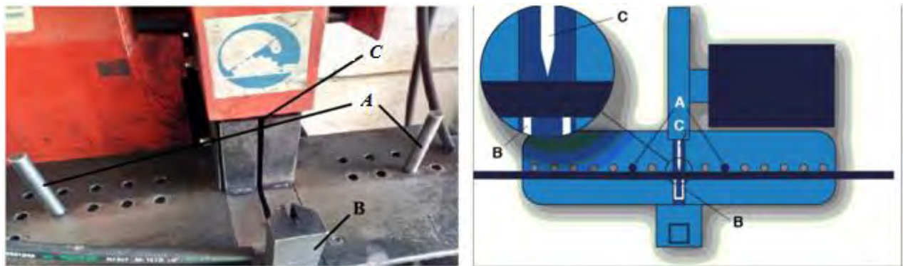
Fig. 5. Basic configuration scheme of hand cutting machine
