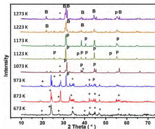
Fig. 2. XRD patterns of the \text{BaFe}_{0.9}\text{Al}_{0.1}\text{O}_{3-\delta} powder calcined at different temperatures: \text{BaCO}_3 (+); \text{BaFe}_2\text{O}_4 (*); hexagonal phase (P) and rhombohedral phase (B)
