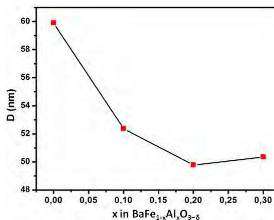
Fig. 7. Crystallite size of \text{BaFe}_{1-x}\text{Al}_x\text{O}_{3-\delta} ( 0.0 \leq x \leq 0.3 ) samples
