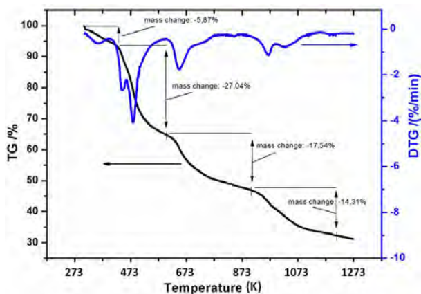
Fig. 1. Thermogravimetric profiles of \text{BaFe}_{0.9}\text{Al}_{0.1}\text{O}_{3-\delta} precursor heated in air at 10 \text{ K min}^{-1}
