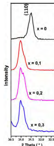
Fig. 4. Evolution of the position of the highest X-ray diffraction peak
