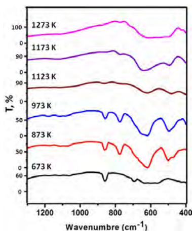
Fig. 6. Infrared spectra of \text{BaFe}_{0.9}\text{Al}_{0.1}\text{O}_{3-\delta} calcined at different temperatures
