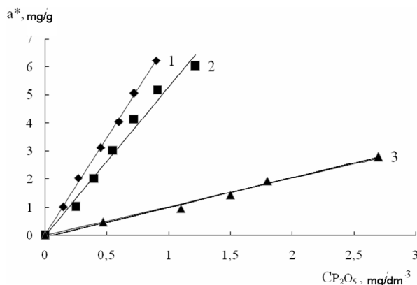
Fig. 4. Isotherms of phosphates, ( \text{KH}_2\text{PO}_4 ) adsorption on natural zeolite (1), jointly with ammonium nitrogen (2), jointly with ammonium nitrogen and albumin (3)
