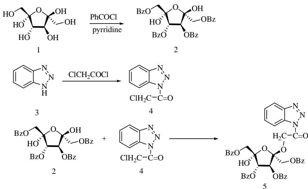
Scheme 1. Total synthesis of nucleoside analogue 5
