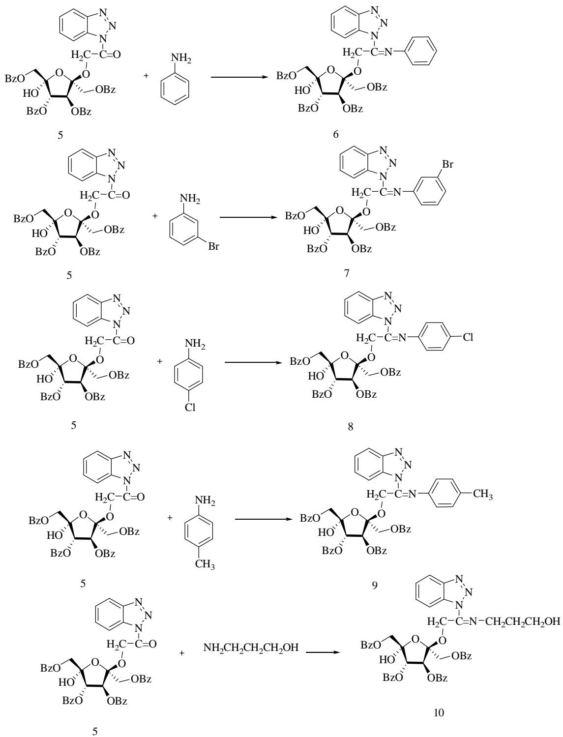
Scheme 3. Formation of Schiff bases 6-10 from nucleoside analogue 5
