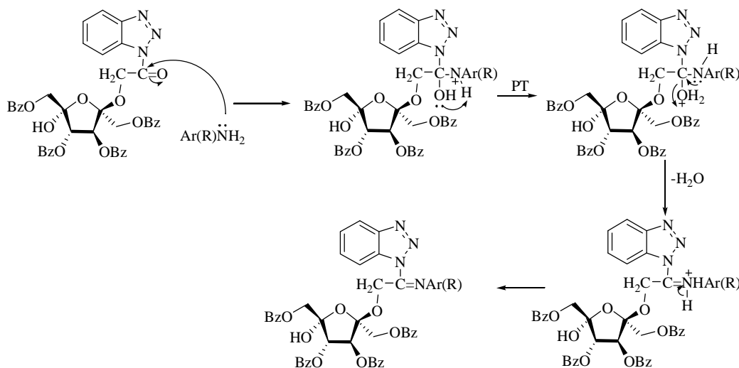
Scheme 4. Mechanism of formation of Schiff bases 6-10
