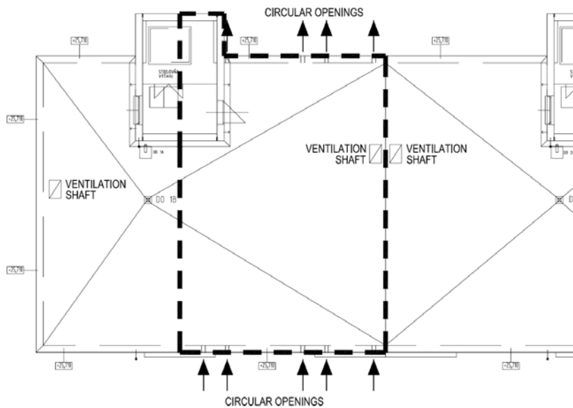
Fig. 1. The top view on the flat roof
