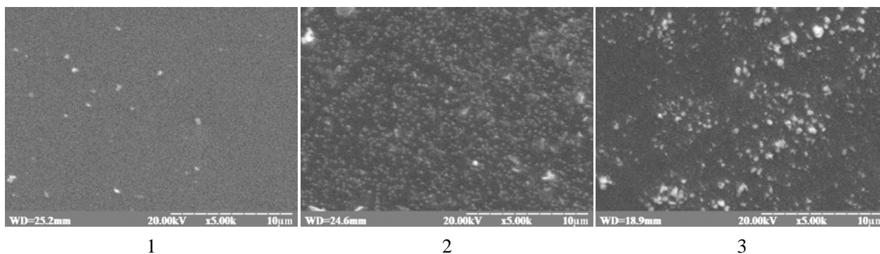
Fig. 4. SEM surface morphology of ZnS films and calculated histogram of the crystal grains height deposited with using various complexing agents: \text{Na}_3\text{C}_6\text{H}_5\text{O}_7 (1); \text{NaOH} (2) and \text{N}_2\text{H}_4\cdot\text{H}_2\text{O}/\text{NH}_3\cdot\text{H}_2\text{O} (3)
