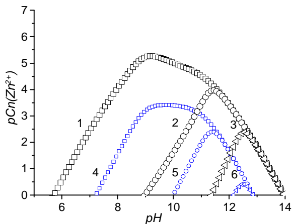
Fig. 1. Boundary conditions of ZnS and Zn(OH)_2 formation in the system Zn^{2+} - L_x - (NH_2)CS , where L_x – trisodium citrate (regions limited by curves 1 and 4, respectively); L_x – ammonia/hydrazine hydrate (regions limited by curves 2 and 5, respectively); L_x – sodium hydroxide (regions limited by curves 3 and 6, respectively)
