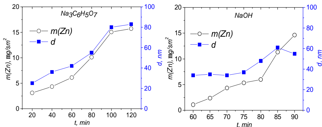
Fig. 6. Dependence of zinc mass change in the ZnS films and their thickness on deposition time ( C(\text{Na}_3\text{C}_6\text{H}_5\text{O}_7) = 0.04 \text{ M} and C(\text{NaOH}) = 0.8 \text{ M} )
