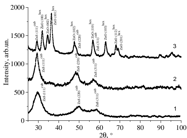
Fig. 2. Experimental profiles of diffractograms of ZnS films obtained using various complexing agents: trisodium citrate (1); sodium hydroxide (2) and hydrazine hydrate/ammonia (3)
