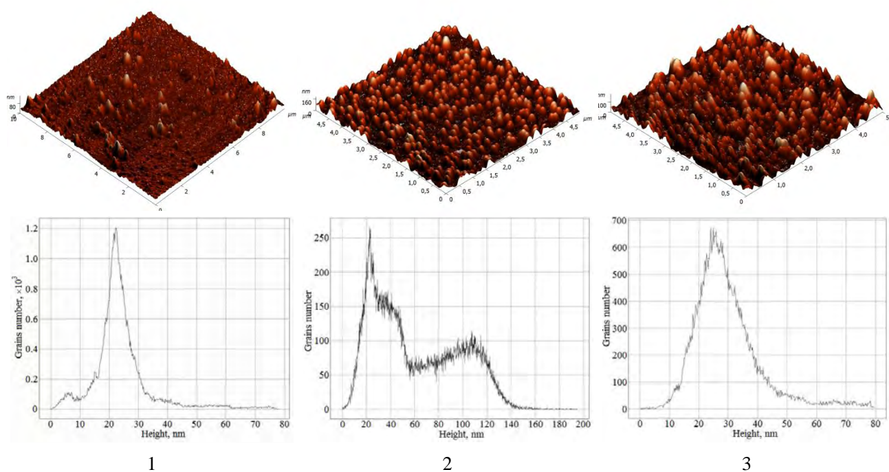
Fig. 5. AFM surface morphology of ZnS films and calculated histogram of the crystal grains height deposited with using various complexing agents: \text{Na}_3\text{C}_6\text{H}_5\text{O}_7 (1); \text{NaOH} (2) and \text{N}_2\text{H}_4\cdot\text{H}_2\text{O}/\text{NH}_3\cdot\text{H}_2\text{O} (3)
