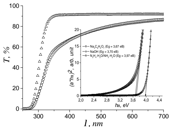
Fig. 3. Spectral dependences of optical transmission ( T , %) of ZnS films synthesized using various complexing agents on glass substrates. Dependence (\alpha \cdot h\nu)^2 = f(h\nu) is on the inset, where \alpha – optical absorption coefficient
