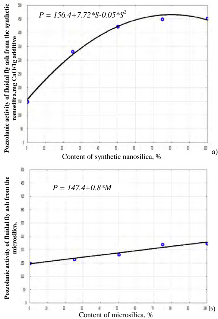
Fig. 3. Models of regression function for the dependence of pozzolanic activity on content of synthetic nanosilica (a) and microsilica (b). For the formula: P – pozzolanic activity; S – content of synthetic nanosilica; M – content of microsilica
