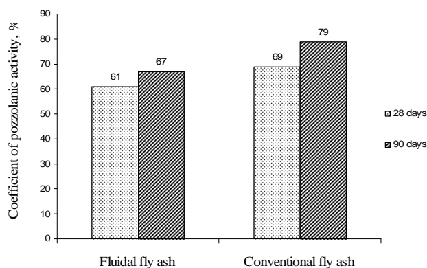
Fig. 1. The coefficient of pozzolanic activity of cement mortar with fluidal and conventional fly ash for 28 and 90 days
