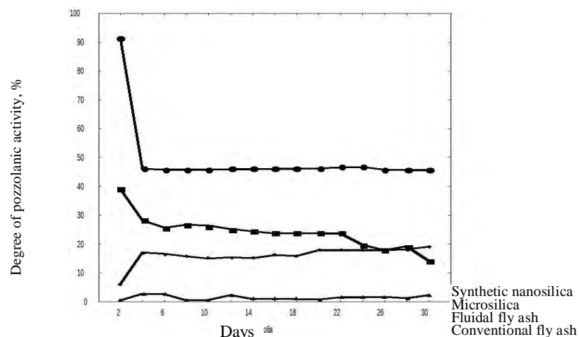
Fig. 2. Degree of pozzolanic activity of the mineral additives
