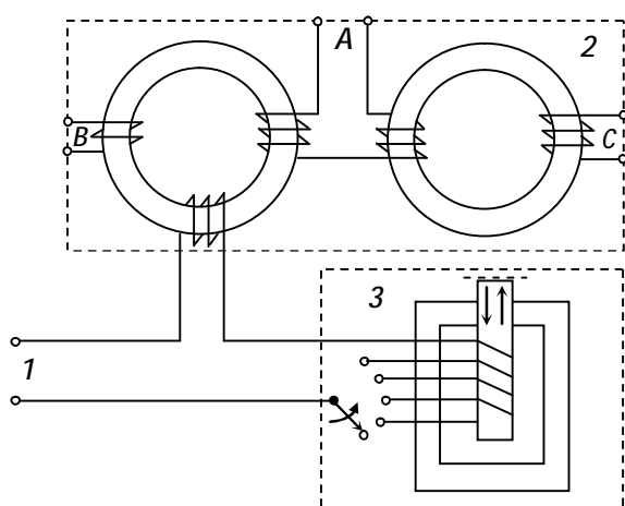
Fig. 3. Diagram of principal part of testing system applied for generation of high alternating currents:
