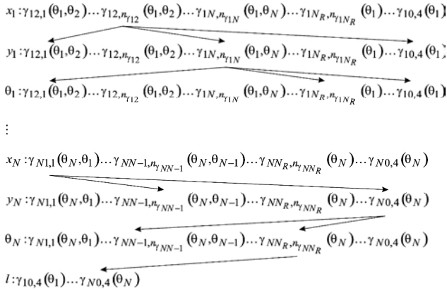
Fig. 4. Solution tree
