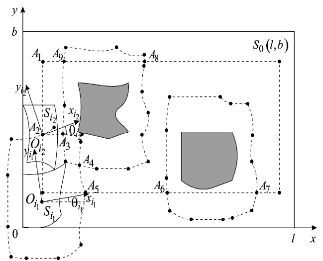
Fig. 5. Placement of object S_{i_2}(x_{i_2}, y_{i_2}, q_{i_2})
