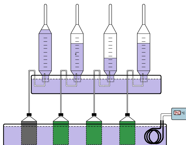
Fig. 1. Laboratory plant for the study of biogas production
