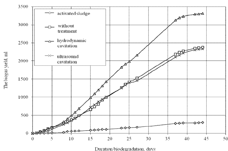
Fig. 2. Biodegradation kinetics of activated sludge and biomass of cyanobacteria under mesophilic conditions
