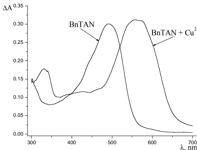
Fig. 3. Molecular absorbance spectra of 1-(5-benzylthiazol-2-yl)azaphthalen-2-ol toluene solutions in the absence and presence of Cu^{2+} ions; C(BnTAN) = 2.32 \cdot 10^{-5} \text{ mol} \cdot \text{l}^{-1} ; C(Cu^{2+}) = 1.16 \cdot 10^{-4} \text{ mol} \cdot \text{l}^{-1} ; C(NaOH) = 0.80 \text{ mol} \cdot \text{l}^{-1} ; l = 1.0 \text{ cm}
