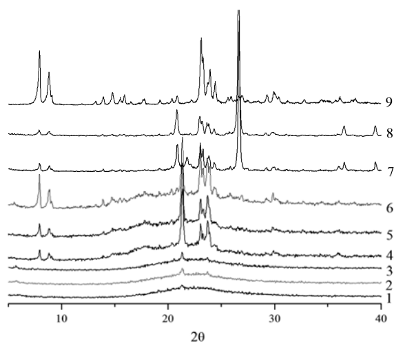
Fig. 2. Samples diffractogram at different hydrothermal temperature and time: 353 K, 11 h (1); 353 K, 24 h (2); 353 K, 48 h (3); 393 K, 11 h (4); 393 K, 24 h (5); 393 K, 48 h (6); 448 K, 24 h (7) and 448 K, 48 h (8). Reference sample of ZSM-5 (9) is given for the comparison
