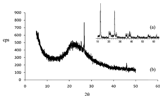
Fig. 1. XRD analysis of uncalcined (a) kaolin (Ref.[23]) and calcined kaolin (metakaolin) (b)
