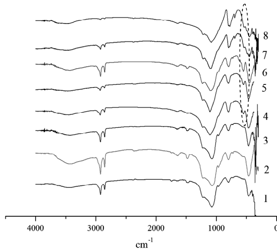
Fig. 3. FT-IR spectra of samples at different hydrothermal temperature and time: 353 K, 11 h (1); 353 K, 24 h (2); 353 K, 48 h (3); 393 K, 11 h (4); 393 K, 24 h (5); 393 K, 48 h (6); 448 K, 24 h (7) and 448 K, 48 h (8)
