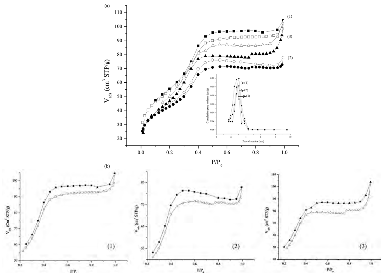
Fig. 4. N 2 adsorption/desorption isotherms (a) and hysteresis loop (b) of the samples at different hydrothermal temperature and time: 393 K, 11 h (1); 393 K, 24 h (2) and 393 K, 48 h (3)
