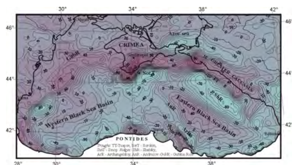
Fig. 1. Simplified anomaly gravity map of the Black Sea region: free-air anomalies (at sea) and Bouguer anomalies (on land). Contour interval is 10 mGal
