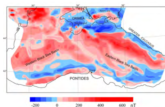
Fig. 2. The anomalous magnetic field \Delta T of the Black Sea
