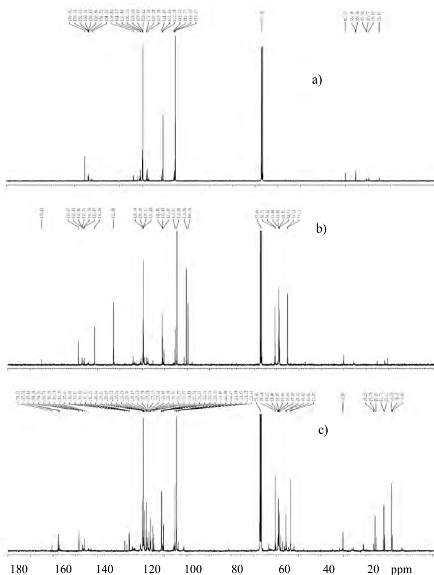
Fig. 5. 13 C NMR spectra of PhFO (a), oligomer I (b) and oligomer II (c)
