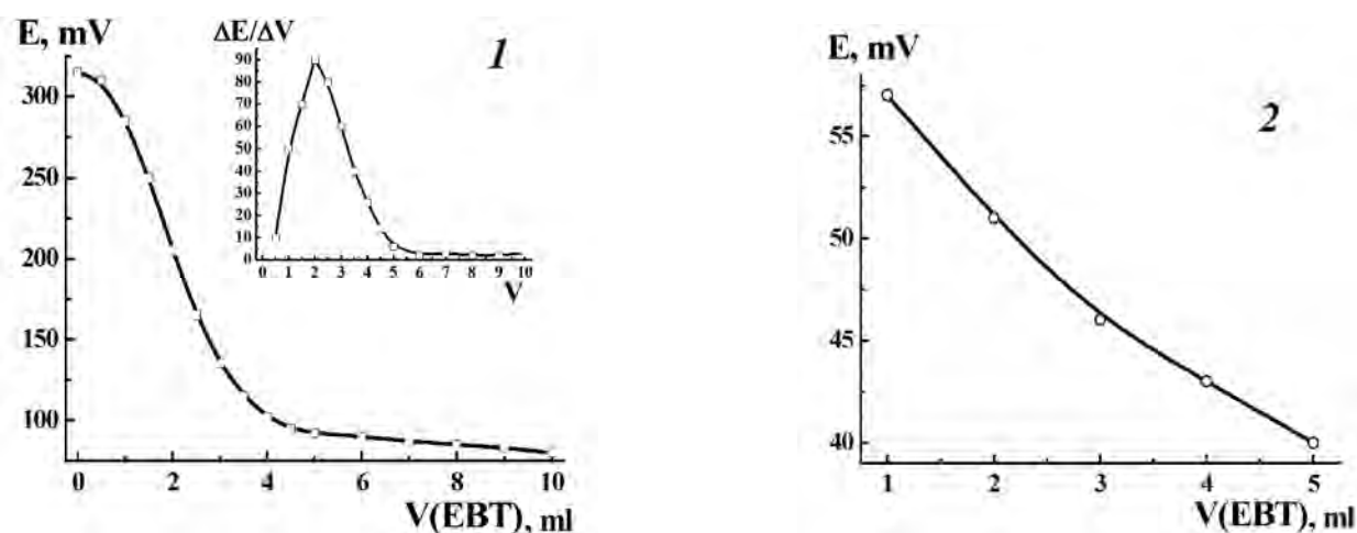
Fig. 5. Curves of the redox titration of SMZ diazonium salt (1) and blank solution (2) by the EBT solution. C_{\text{HCl}}=1.0\text{ M} , C_{\text{SMZ}}=1.75\cdot 10^{-3}\text{ M} , C_{\text{NaNO}_2}=1.75\cdot 10^{-2}\text{ M} , C_{\text{Urea}}=0.875\text{ M} , C_{\text{EBT}}=1.75\cdot 10^{-3}\text{ M} , C_{\text{UBM}}=4.0\cdot 10^{-3}\text{ M}
