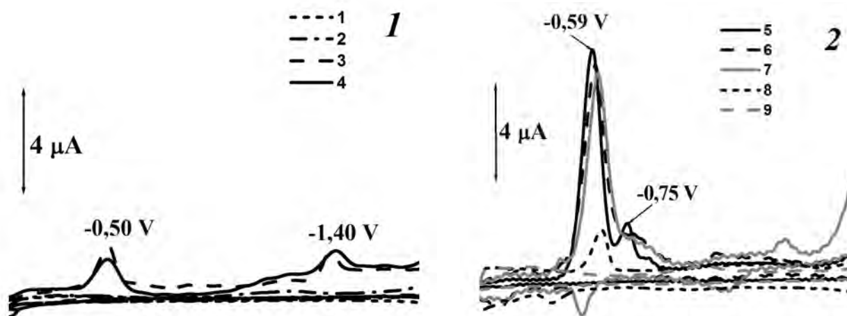
Fig. 6. Polarograms of the reduction processes: Urea (1), \text{NO}_2^- (2), SMZ (3), \text{SMZ}+\text{NO}_2^- (4), EBT (5), \text{NO}_2^- +EBT (6), (\text{SMZ}+\text{NO}_2^-+\text{Urea})+\text{EBT} (7), \alpha -naphthol (8), (\text{SMZ}+\text{NO}_2^-+\text{Urea})+\alpha -naphthol (9). C_{\text{HCl}}=1.0\text{ M} , C_{\text{SMZ}}=6.0\cdot 10^{-5}\text{ M} , C_{\text{NaNO}_2}=8.0\cdot 10^{-4}\text{ M} , C_{\text{Urea}}=4.0\cdot 10^{-2}\text{ M} , C_{\text{EBT}}=3.6\cdot 10^{-4}\text{ M} , C_{\text{UBR}}=4.0\cdot 10^{-3}\text{ M} , \text{pH}=8.0
